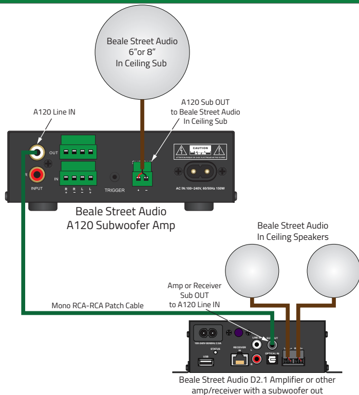
LINE LEVEL INPUT ILLUSTRATION
