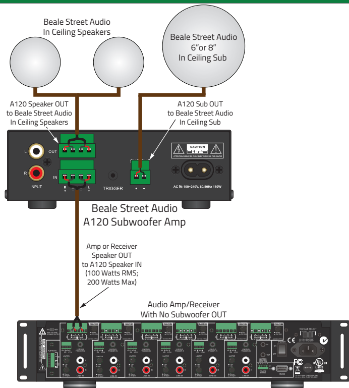
SPEAKER LEVEL INPUT ILLUSTRATION
