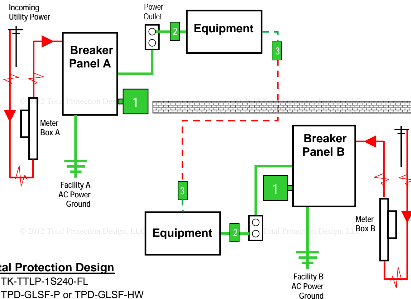
TPD-GLSF-P Plug In Version - 20Amp
