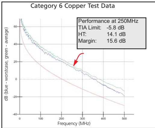
Worst case - 2-connector channel — Test results by Intertek (ETL)
