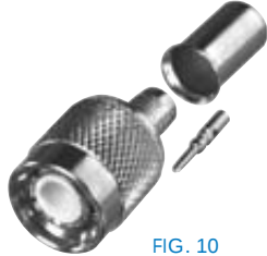
FIG. 10 RFT-1203-1P, -1X
