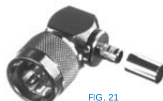
FIG. 21 RFN-1009-X-04
